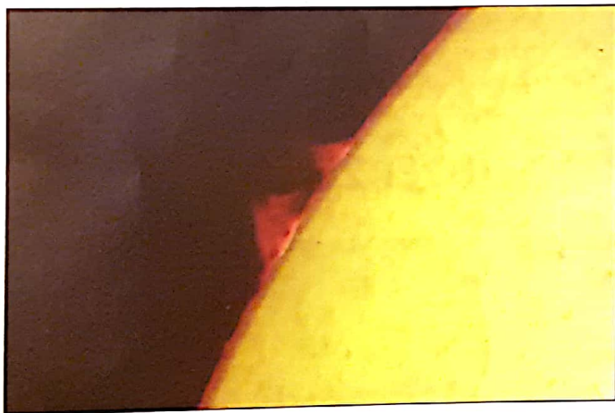
Protuberanca na Soncu
